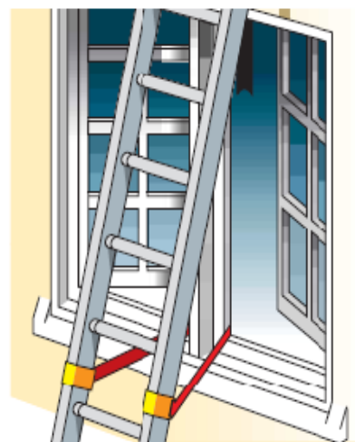
Tying part way down
